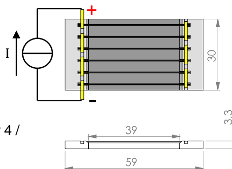
M3930E24 – Actuator Module only
